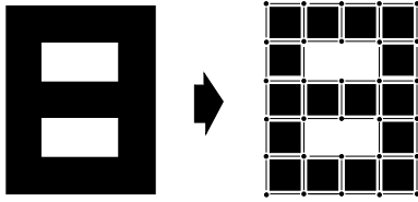
Fig. 1. The disjoint decomposition of a pattern K (left) into a sum \mathcal{P} (right) of disjoint interior elements.
