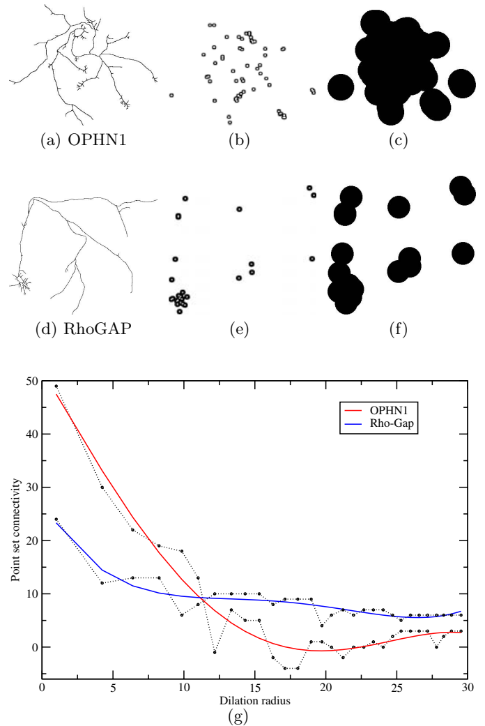
Fig. 2. Isolating morphological information relating to the neuronal branching structure while preserving the metric relationship among the branching points. Each bifurcating point undergoes an exact dilation while its connectivity is recorded as function of the scale parameter. Prototypical transfected rat neuronal cell, a) and d). Extracted pattern of bifurcation points, b) and e). The end of the bifurcation point parallel set dilation procedure, c) and f). The resulting discriminating functional for both neuron types, g).
